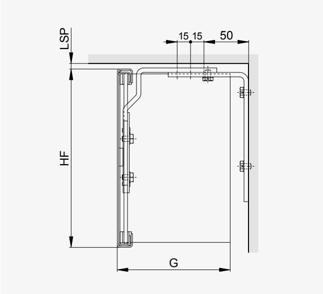
1.1 Straight cover.
