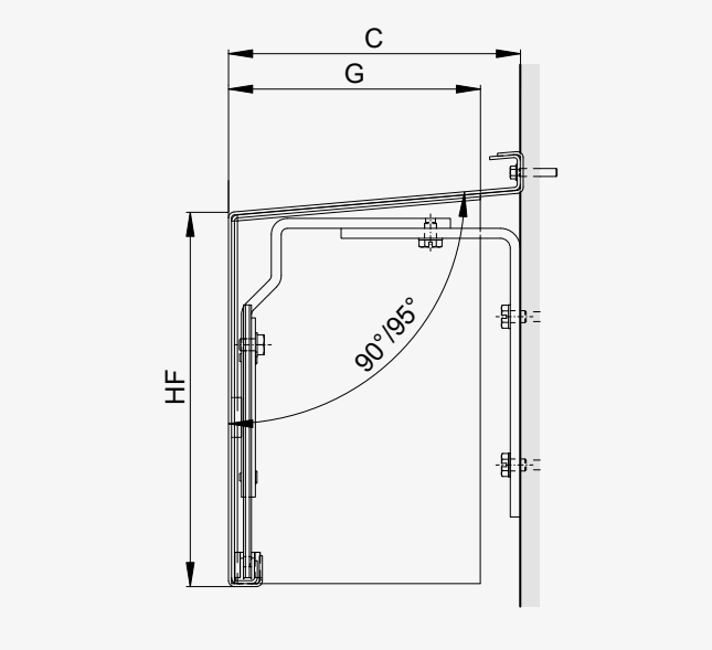
8.1 Porch cover.
